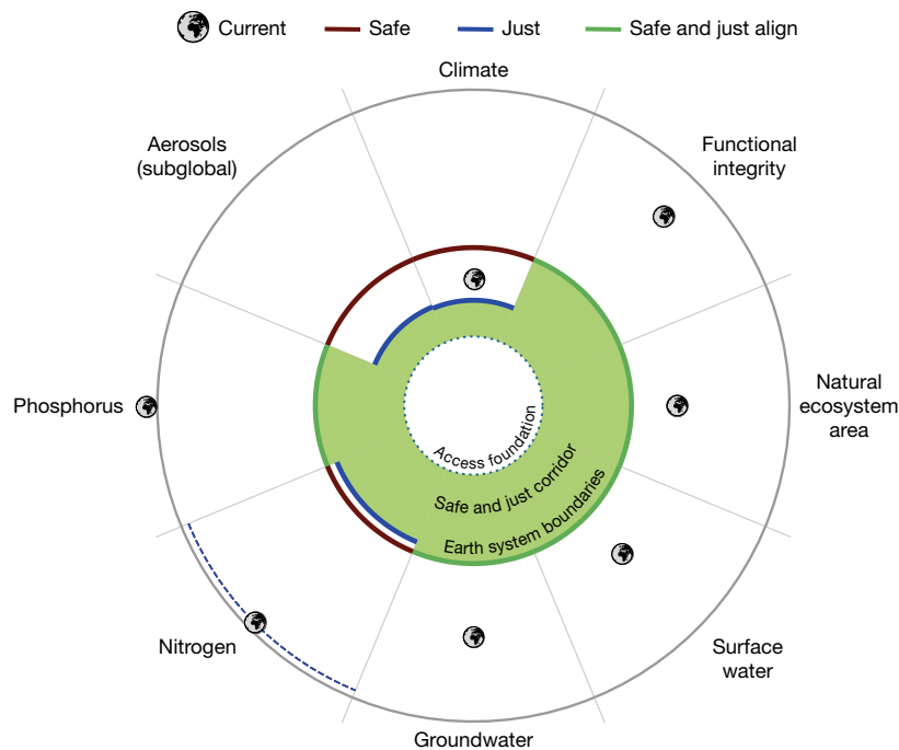
Fig. 1 | Proposed safe and just (NSH) ESBs. Visualization of safe ESBs (dark red), just (NSH) ESBs (blue), cases where safe and just (NSH) boundaries align (green) and current global states (Earth icons). Radial axes are normalized to safe ESBs. Headline or central estimate global boundaries (Table 1) are plotted to support comparison with the current global state, but we emphasize that we have also defined subglobal boundaries and multiple likelihood levels for many domains (Table 1). For aerosols, however, we display the subglobal boundaries to compare safe and just boundaries. For nitrogen, we plot with a dashed blue line the
