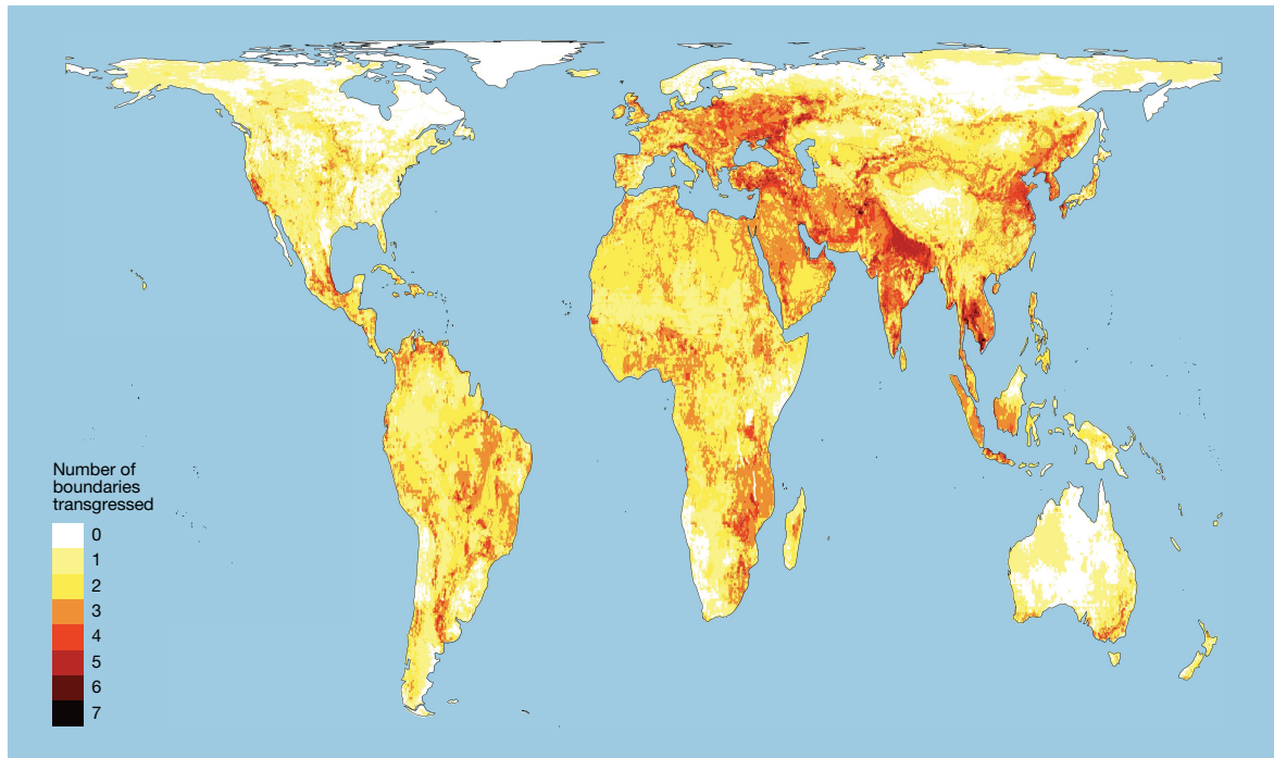
Fig. 3 | Hotspots of current ESB transgressions. The number of subglobal climate (two local exposure boundaries), functional integrity, surface water, groundwater, nitrogen, phosphorus and aerosol safe and just ESBs currently transgressed by location. No more than seven of these eight metrics have their ESBs transgressed in any one pixel. Since climate is a globally defined ESB, we use wet bulb temperatures of over 35 °C for at least 1 day per year and low-
