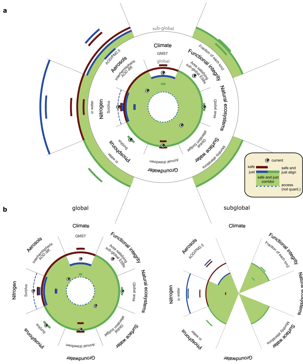
Extended Data Fig. 1 | Alternative visualizations of safe and just Earth system boundaries (Fig. 1). Concentric ( a ) and parallel ( b ) visualizations of global ( a , inner circle; b , left circle) and sub-global ( a , outer circle; b , right circle) safe and just ESBs. Colours are as in Fig. 1. Global rings ( a , inner circle;
