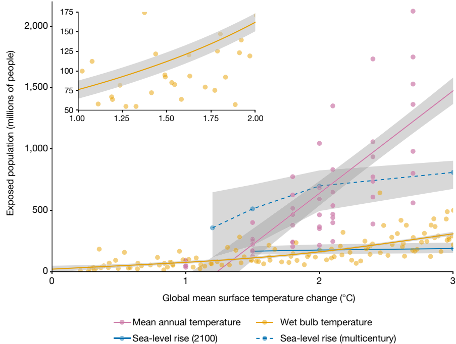
Fig. 2 | Exposure to significant harm from climate change at different levels of warming. We examine the exposure of the 2010 global population to mean annual temperatures above 29 °C (purple; linear fit, P < 0.01 ), wet bulb temperatures of 35 °C for an average of at least 1 day per year (orange; quadratic fit, P < 0.01 ) and future sea-level rise (blue; linear interpolation). Sea-level rise is
